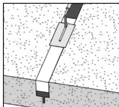
Step 3 Install Krystol Bari-cote™
