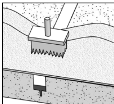
Step 5 Install Krystol T2® slurry coat
