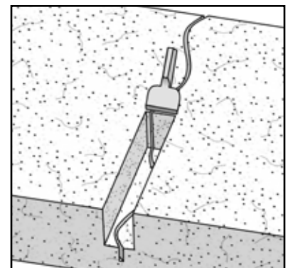
Step 1 Chisel and prepare the crack
