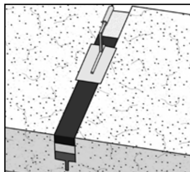
Step 4 Install Krystol Bari-cote™
