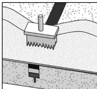
Step 5 Install Krystol T1® & T2® slurry coats
